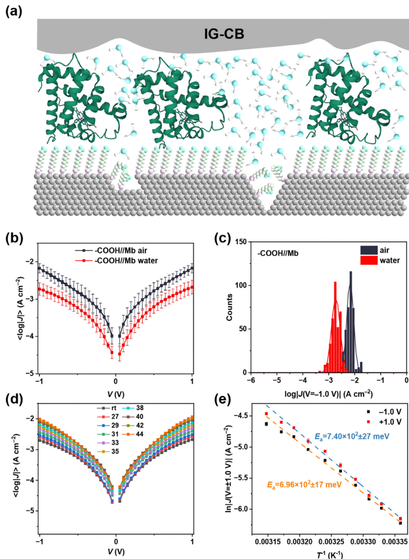
Fig. 4 (a) The scheme of molecular junctions with myoglobin proteins conducted in water. (b) Plots of the \langle \log |J| \rangle curves for Ag TS -SC 10 COOH//Mb//IG-CB junctions tested in air and water. (c) The corresponding histograms of \log |J| at -1.0 V with Gaussian fits. (d) T -dependent \langle \log |J| \rangle data for the junctions of Ag TS -SC 10 COOH//Mb//IG-CB in water. (e) Corresponding Arrhenius plots for \langle \ln |J| \rangle at \pm 1.0 V.
