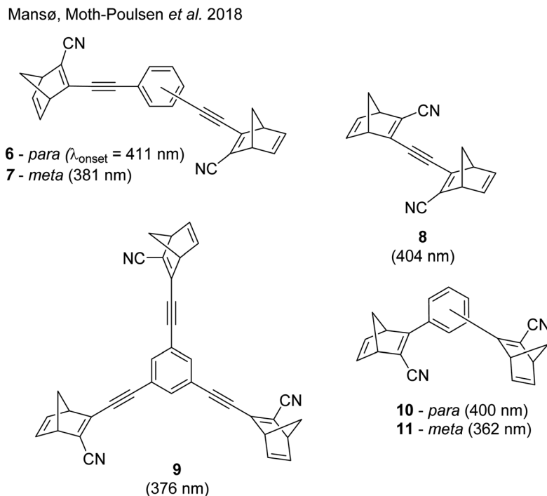
Fig. 3 Structure of the oligomeric NBD units reported by Mansø, Moth-Poulsen et al. , with \lambda_{\text{onset}} values given in parentheses. 13
