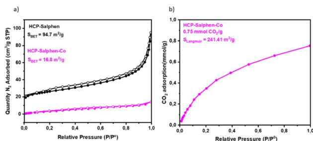
Fig. 4 (a) N_2 adsorption (solid circles)/desorption (open circles) of HCP-Salphen-Co and HCP-Salphen; (b) \text{CO}_2 uptake of HCP-Salphen-Co.
