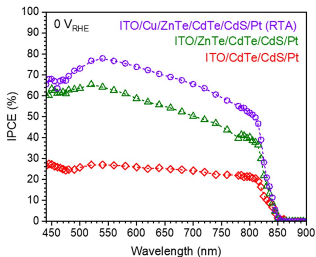
Fig. 7 IPCE spectra obtained from ITO/CdTe/CdS/Pt, ITO/ZnTe/CdTe/CdS/Pt and ITO/Cu/ZnTe/CdTe/CdS/Pt photocathodes at 0 \text{ V}_{\text{RHE}} under monochromatic light. As an electrolyte, a 1 \text{ M} aqueous KPi solution with pH adjusted to 6.5 was employed.
