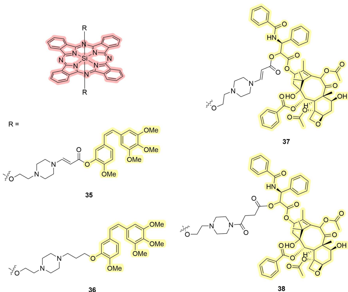
Fig. 11 Structures of silicon phthalocyanines 35 – 38 that exhibit properties of PDT/PACT agents. Red highlights the PS, while yellow indicates the compound released.
