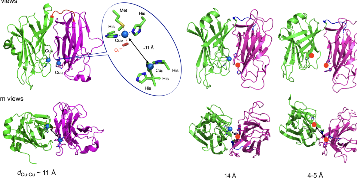
Fig. 2 Uncoupled binuclear copper-containing monooxygenases, PHM and D \beta H. (a) and (b) reactions catalyzed by PHM and D \beta H, respectively; (c) X-ray structure of PHM from Rattus norvegicus showing the two domains (Cu M domain in green and Cu H domain in magenta) connected by a loop (in blue) in which each domain binds a single copper atom spaced from each other by approximately 11 \text{\AA} and (d) structure of the Cu M -superoxido intermediate in PHM (PDB ID 1opm); (e) and (f) X-ray structure of the human D \beta H (PDB ID 4zel) showing the open (e) and the closed (f) forms. Only the Cu M domain of the closed form contains a copper atom, the other copper ions (red sphere) are manually placed.
