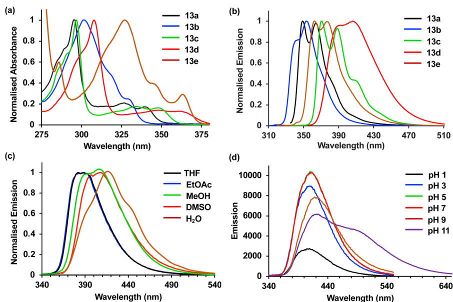
Fig. 3 (a) Absorption spectra of amino acids 13a – 13e (5 \mu M) in methanol. (b) Normalised emission spectra of amino acids 13a – 13e (5 \mu M) in methanol. (c) Normalised emission spectra of 13d (5 \mu M) in various solvents. (d) Emission spectra of 13d (5 \mu M) at various pH.
