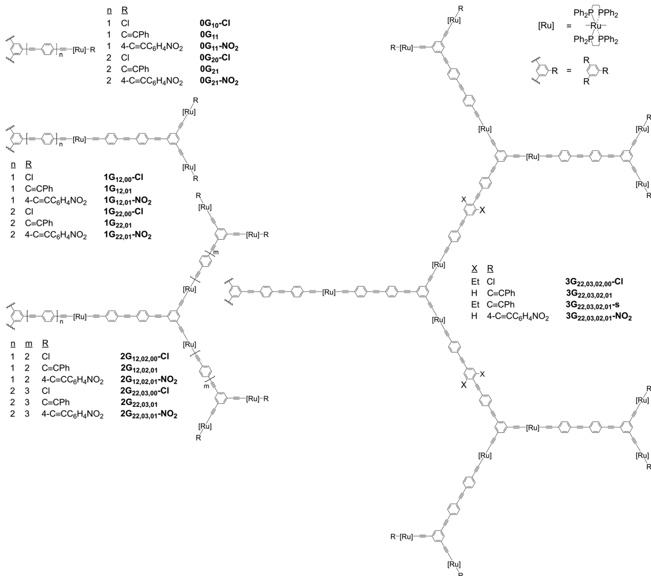
Fig. 1 Organoruthenium dendrimers in this study. [Ru]: \text{trans-[Ru}(\kappa^2\text{-dppe)}_2\text{]} (dppe = 1,2-bis(diphenylphosphino)ethane). Wavy lines: equivalent dendrons at dendrimer cores. Names follow the format: (i) nG ( n -th generation dendrimer), (ii) xy ( x and y phenyleneethynylene units between the branching points and the ligated Ru at each generation level, commencing at the core), (iii) a comma “,” separating the “ xy ” numbers of OPE units at each generation level, and in some cases (iv) –s (installation of solubilizing Et groups at the central phenylene of the OPE unit between the first- and second-generation branching points).
