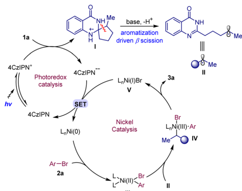
Scheme 4 Proposed Mechanism.
