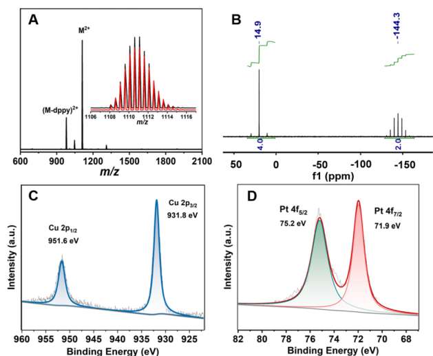
Fig. 1 (a) ESI-MS spectra of MeO-Cu 4 Pt 2 . M = [\text{Cu}_4\text{Pt}_2(\text{MeO}-\text{PhC}\equiv\text{C})_4(\text{dppy})_4]^{2+} . (b) ^{31}\text{P} NMR spectrum of the MeO-Cu 4 Pt 2 . (c) Cu 2p and (d) Pt 4f XPS data for MeO-Cu 4 Pt 2 .
