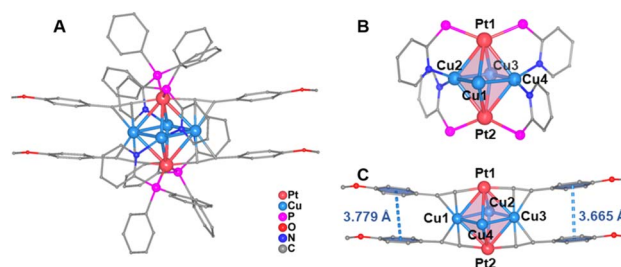
Fig. 2 (a) The total crystal structure of MeO-Cu 4 Pt 2 . (b) Coordination motif of two dppy ligands. The benzene rings in dppy are omitted for clarity. (c) Bridging mode of four \text{MeO}-\text{PhC}\equiv\text{C}^- ligands highlighting two pairs of \pi\cdots\pi interactions between the benzene rings of alkynyl groups.
