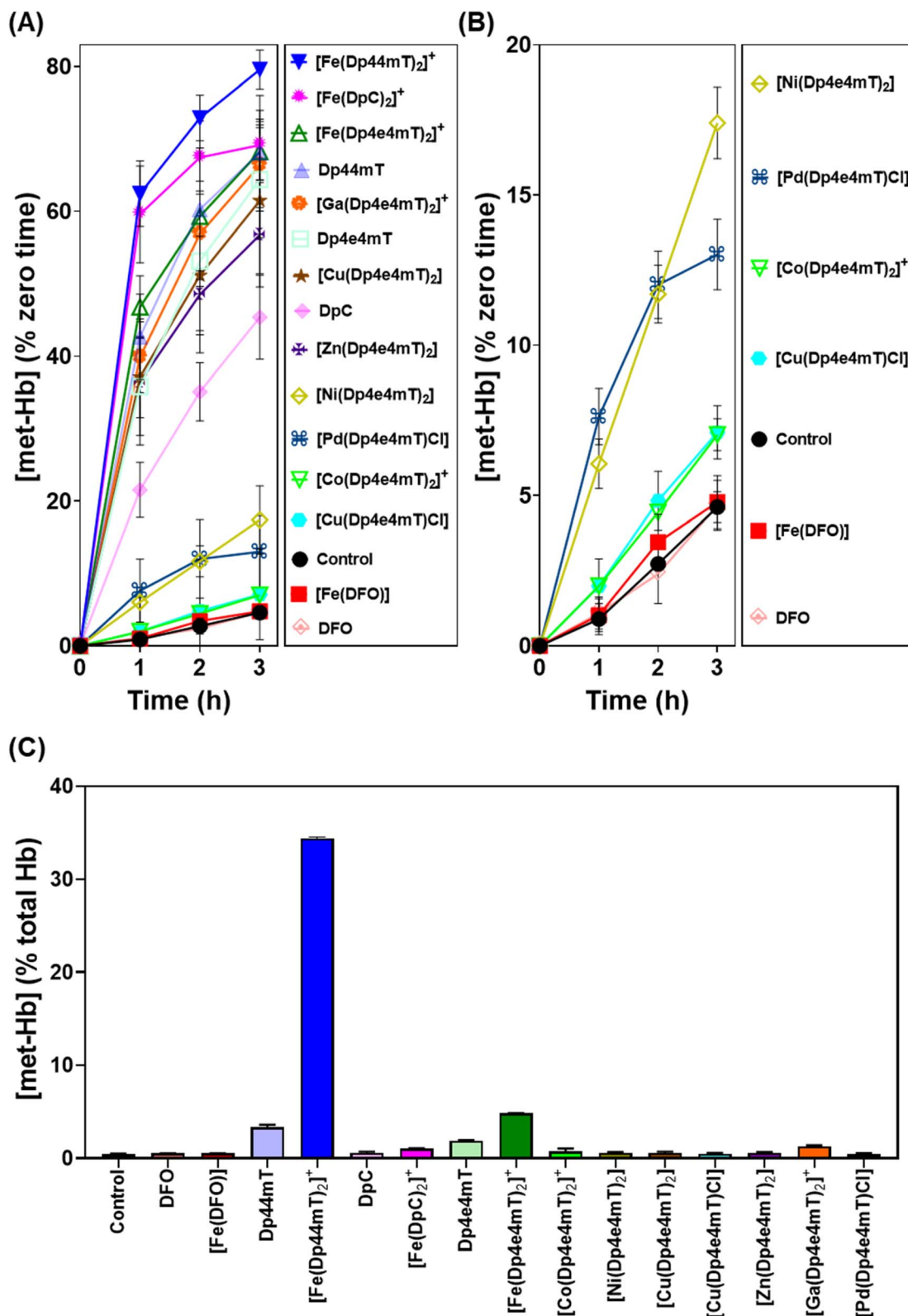
Fig. 7 (A and B) Investigation of the effects of \text{Dp4e4mT} and its \text{Fe}(\text{III}) , \text{Co}(\text{III}) , \text{Ni}(\text{II}) , \text{Cu}(\text{II}) , \text{Zn}(\text{II}) , \text{Ga}(\text{III}) , and \text{Pd}(\text{II}) complexes versus DFO, \text{Dp44mT} , \text{DpC} and their \text{Fe}(\text{III}) complexes ( 10 \mu\text{M} ) on met-Hb generation (% zero time) after an incubation of 1–3 h/ 20^\circ\text{C} with purified oxy-Hb ( 40 \mu\text{M} ). (C) Investigation of the effects of \text{Dp4e4mT} and its \text{Fe}(\text{III}) , \text{Co}(\text{III}) , \text{Ni}(\text{II}) , \text{Cu}(\text{II}) , \text{Zn}(\text{II}) , \text{Ga}(\text{III}) , or \text{Pd}(\text{II}) complexes relative to the positive controls DFO, \text{Dp44mT} , \text{DpC} , and their \text{Fe}(\text{III}) complexes ( 10 \mu\text{M} ) on oxy-Hb oxidation in intact human erythrocytes after a 3 h/ 37^\circ\text{C} incubation. Results are mean \pm SD (3 experiments).
