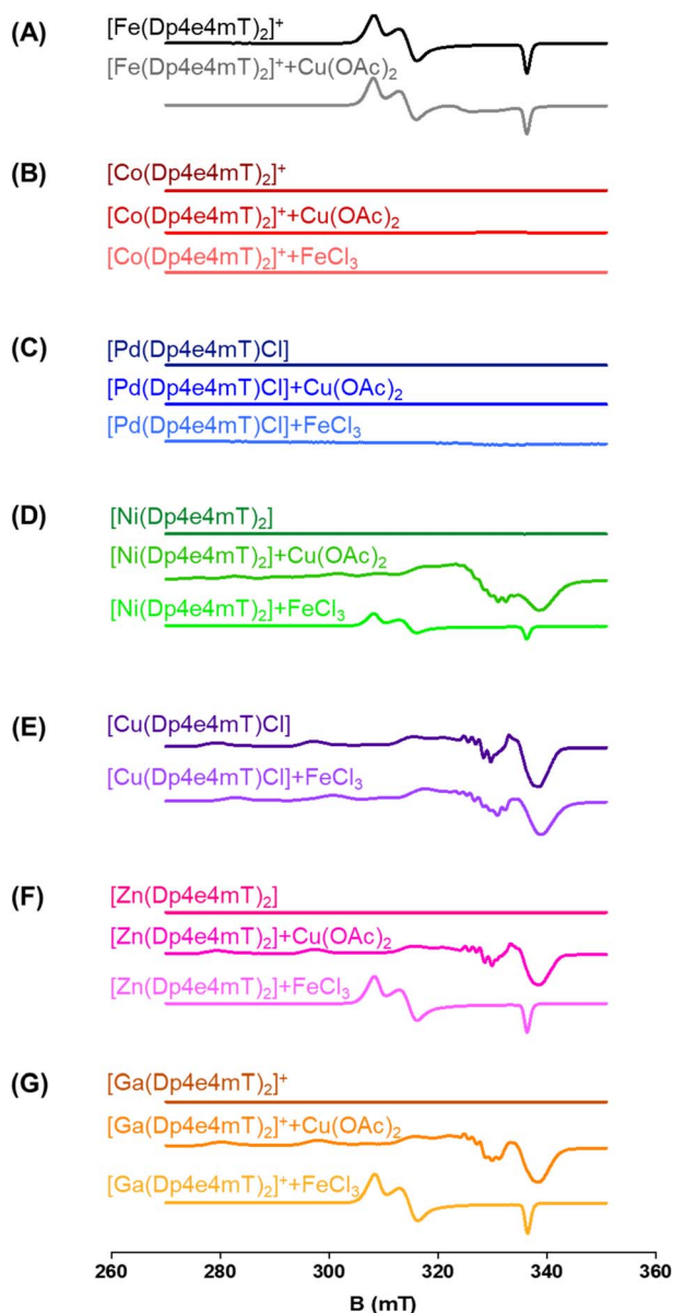
Fig. 3 (A–G) The transmetallation of the Dp4e4mT complexes was examined using X-band CW EPR spectroscopy. The complexes (500 \mu M in DMSO : CHCl 3 1 : 1) and their products after reaction with equimolar amounts of Cu(OAc) 2 and FeCl 3 after a 24 h/20 °C incubation.
