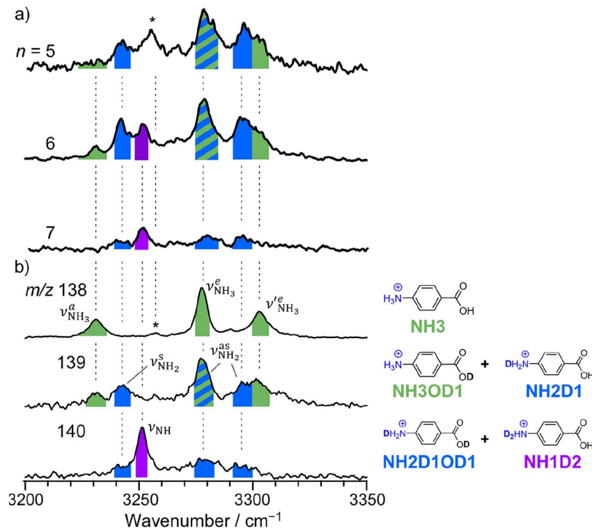
Fig. 3 (a) CAS-IRPD spectra of \text{PABAHD}^+(\text{D}_2\text{O})_n ( n = 5-7 ) in the 3200-3350 \text{ cm}^{-1} range (reprinted from the inset spectra in Fig. 2). (b) IRPD spectra of \text{PABAHD}^+ ( m/z 138), singly deuterated protonated PABA ( m/z 139), and doubly deuterated protonated PABA ( m/z 140). These spectra are necessary to assign the CAS-IRPD spectra because the monomer core after the CAS event includes several deuterated isotopomers. The green-, blue-, and purple-colored bands are assigned to NH stretches of \text{NH}_3 , \text{NH}_2\text{D}_1 , and \text{NH}_1\text{D}_2 , respectively. The band marked by an asterisk is assigned to a combination band of the O-protomer (in-plane \text{NH}_2 bend 24,44 at \sim 1660 \text{ cm}^{-1} + aryl C-C stretch 24,44 at \sim 1600 \text{ cm}^{-1} ). This type of combination band is also observed for an analog of PABA, ethyl p -aminobenzoate. 43
