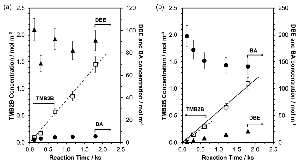
Fig. 3 Liquid-phase concentrations of TMB2B ( \square ), BA ( \bullet ) and DBE ( \blacktriangle ) as a function of batch reaction time during mesitylene benzylation (363 K) with (a) DBE (TMB:DBE molar ratio = 75:1; DBE/Al molar ratio = 25) or (b) BA (TMB:BA molar ratio = 40:1; BA/Al molar ratio = 23) on MFI-40-P. Dashed lines represent the best-fit line of the TMB2B concentration vs. time at short reaction times. Solid line in 3(b) represents the best fit line of the TMB2B concentration vs. time at all reaction times. Uncertainties in measured concentrations are \pm 10\% .
