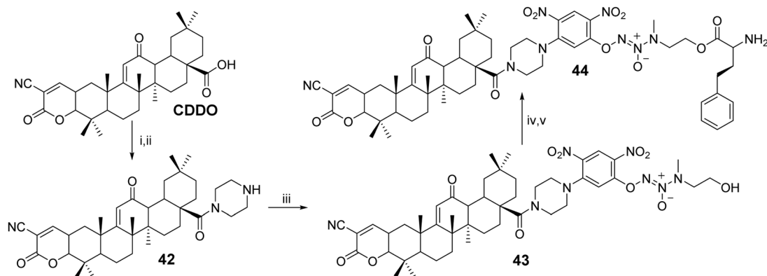
Fig. 13 Synthesis of OA derivatives 42 to 44.
