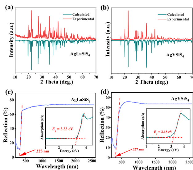
Fig. 4 The experimental and calculated XRD patterns of (a) \text{AgLaSiS}_4 and (b) \text{AgYSiS}_4 ; the UV-vis-NIR diffuse reflectance spectra and experimental band gaps of (c) \text{AgLaSiS}_4 and (d) \text{AgYSiS}_4 .
