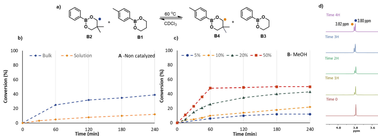
Fig. 4 (a) Experimental kinetics of the reaction between dioxaborinane B2 and B1 at 60 °C for 4 hours. (b) Kinetics of B2 + B1 without catalyst in solution ( \text{CDCl}_3 ) and in bulk. (c) Kinetics of B2 + B1 in solution with 5, 10, 20 and 50 mol% of MeOH with respect to the dioxaborinanes. (d) Time-dependent ^1\text{H} -NMR spectra of the bulk kinetic reaction of the two dioxaborinanes.
