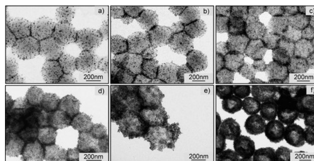
Fig. 12 Transmission electron microscopy (TEM) images of the MagNanogels synthesised by Cortes et al. with different IONPs content (from a to f: 9.0, 16.7, 28.6, 37.5, 50.0, and 66.7 wt%). 113 Reprinted with permission from E. Cazares-Cortes et al. , ACS Appl. Mater. Interfaces 2017, 9, 31, 25775–25788. Copyright 2017 American Chemical Society.
