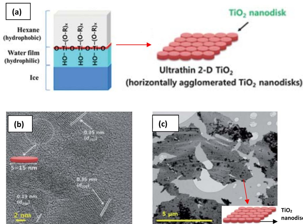
Fig. 8 (a) Schematic illustration of the 2-D TiO 2 formation on the hexane/ice interface. 84 TEM images of a nanosheet consisting of horizontally agglomerated TiO 2 nanodisks. 84 (b) HR-TEM image of nanodisks, (c) TEM image of nanosheets. Reproduced from ref. 84 with permission from the Royal Society of Chemistry.
