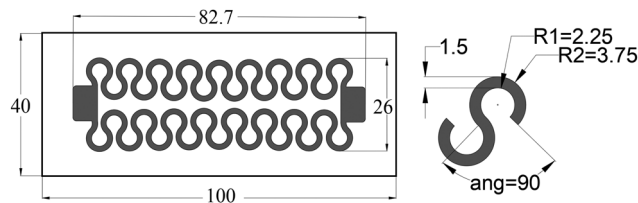
Fig. 2 Respiratory rate sensor design. The figure on the left shows the full sensor CAD design inside a 100 \times 40 mm substrate, while the figure on the right shows the dimensions of a single horseshoe waveform that is repeated across the length of the sensor.
