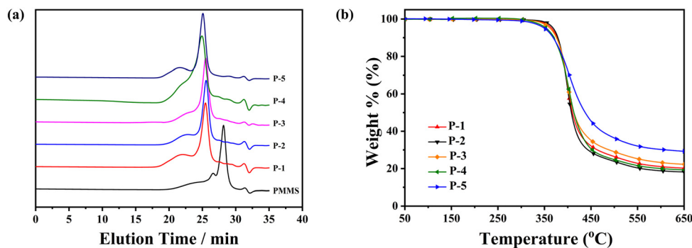
Fig. 2 (a) GPC spectra of all the polymers and PMMS and (b) TGA traces of polymers in nitrogen at a rate of 20\text{ }^{\circ}\text{C min}^{-1} .
