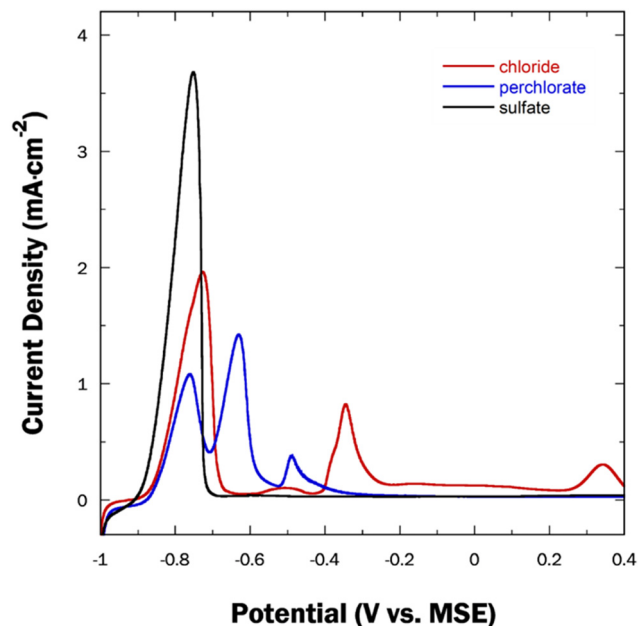
Fig. 9 LSV curves depicting the oxidation of Cu_{22.6}Sn_{77.4} alloys in different dealloying baths; the precursor alloys were prepared on Au substrates and were dealloyed at \nu = 1 mV s^{-1} . The corresponding arrows indicate the potential cut-offs for dealloying.
