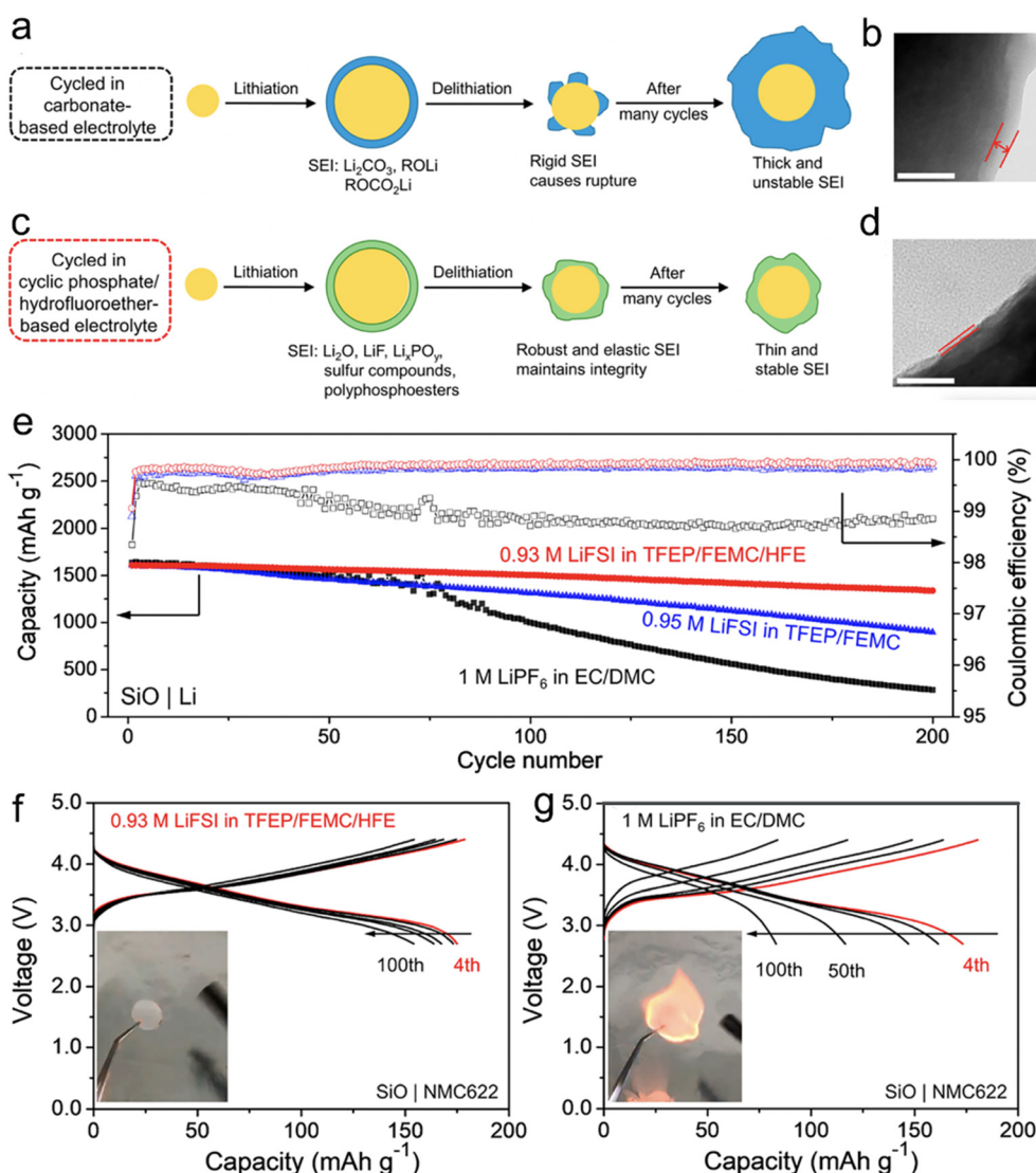
Fig. 4 Schematic illustrations of SEIs on an SiO particle derived from (a) 1 M \text{LiPF}_6 in EC/DMC and (c) 0.93 M \text{LiFSI} in TFEP/FEMC/HFE (in the conventional EC based electrolyte, an SEI mainly consisting of \text{Li}_2\text{CO}_3 , \text{ROCO}_2\text{Li} , and \text{ROLi} forms at the first lithiation, which is too rigid to tolerate the volumetric stress during delithiation. On the other hand, the SEI generated by the cyclic phosphate/hydrofluoroether-based electrolyte is mainly composed of \text{Li}_2\text{O} , \text{LiF} , \text{Li}_x\text{PO}_y , sulfur compounds, and polyphosphoesters, which is highly elastic and robust and can sustain the volume changes of SiO upon cycling); TEM images of the SiO electrodes after cycling in (b) 1 M \text{LiPF}_6 in EC/DMC and (d) 0.93 M \text{LiFSI} in TFEP/FEMC/HFE for 100 cycles (the distance between two lines represents the thickness of the SEI, which clearly shows that the SEI formed in 0.93 M \text{LiFSI} in TFEP/FEMC/HFE is much thinner than that in 1 M \text{LiPF}_6 in EC/DMC electrolyte. The white scale bar represents 50 nm); (e) cycling performance of the SiO|Li half-cells using 0.93 M \text{LiFSI} in TFEP/FEMC/HFE, 0.95 M \text{LiFSI} in TFEP/FEMC, and 1 M \text{LiPF}_6 in EC/DMC at 0.2C after three formation cycles at 0.05C; selected charge-discharge curves for the full cells at 0.4C with (f) 0.93 M \text{LiFSI} in TFEP/FEMC/HFE and (g) 1 M \text{LiPF}_6 in EC/DMC (the capacity is based on the weight of the NMC622 active material. The insets show the flammability test results). Reprinted with permission from ref. 74. Copyright 2021, American Chemical Society.
