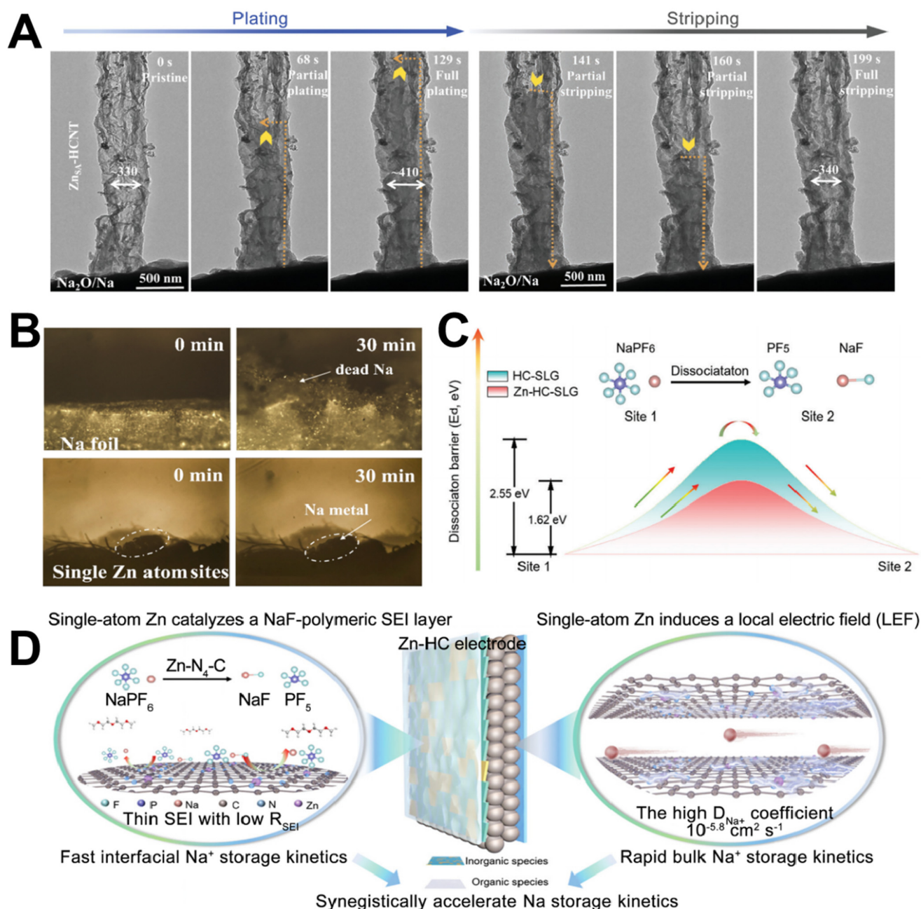
Fig. 8 (A) In situ TEM observation of metallic Na plating/stripping on the \text{ZnSA-HCNT} anode. 69 Copyright 2022, Wiley-VCH. (B) In situ optical microscopy observations. Reproduced with permission. 70 Copyright 2019, American Chemical Society. (C) Dissociation energy barrier of HC-SLG with/without SAZn to catalyze \text{NaPF}_6 . (D) Schematic of the Zn-HC-enhanced rate capability mechanism. Reproduced with permission. 71 Copyright 2023, Wiley-VCH.
