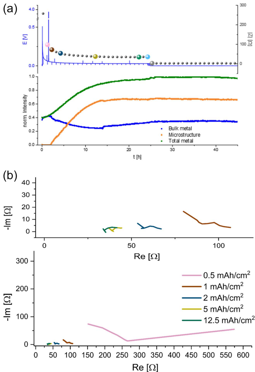
Fig. 9 (a) Operando ^7\text{Li} NMR and impedance (GEIS) measured at 9 Hz. Intensities measured during unidirectional Li plating at 1 \text{mA cm}^{-2} in an NMR in situ cylindrical symmetrical Li cell with LP30 + 10% FEC electrolyte. (b) GEIS Nyquist plots measured with 100 \mu\text{A} amplitude during Li plating at 1 \text{mA cm}^{-2} in an NMR in situ cylindrical symmetric cell, using LP30 + FEC electrolyte with GF separator at RT. Magnification of the plot at 5–15 \text{mA h cm}^{-2} .
