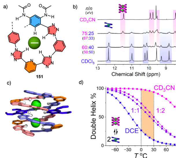
Fig. 73 (a) Chemical structure of anion foldamer host 151 . (b) Double helix formation of 151 -Cl - in response to solvent polarity (5 mM, 15 equiv. of TEACl). (c) DFT-optimized geometry of the 2 : 2 double helix formed by 151 -Cl. (d) Two factors combined showing maximal solvent-induced swings in double helix population around ambient temperatures (orange shade). Reproduced from ref. 357 with permission from the American Chemical Society, copyright 2018.
