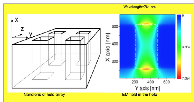
Fig. 35 (Left) thin film with holes working as a nanolens. (Right) the enhanced electric field at the top and bottom of a hole. Courtesy of Dr. Ying Fu
