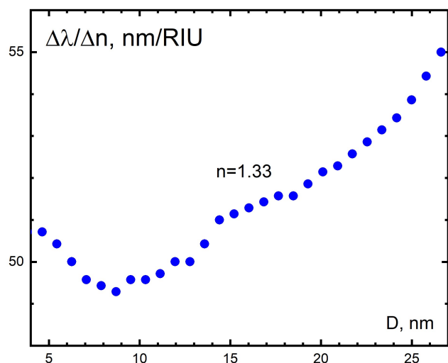
Fig. 23 Dependence of the refractive index sensitivity (RIS) of Au nanoparticles with sizes 5–27 nm at the refractive index of aqueous medium ( n=1.33 ). The Mie theory calculations with size correction for the Au dielectric constants by Karimi 130 . From Ref. 124
