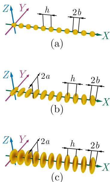
Fig. 37 Schematic representation of chained plasmonic nanoparticle waveguides consisting of (a) spheres, (b) prolate spheroids, and (c) oblate spheroids. Reproduced from Ref. 243 with permission from Elsevier, copyright 2018.
