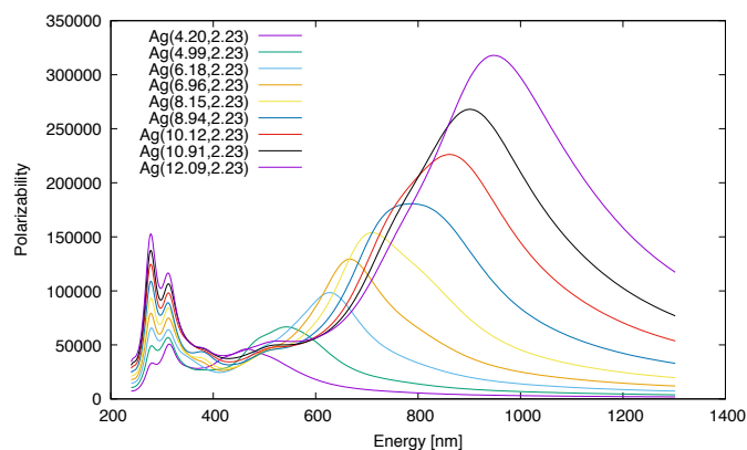
Fig. 5 Polarizability versus incident energy for Ag(x,2.23) nanorods with different longitudinal plasmon lengths. Reproduced from Ref. 75 with permission from ACS, copyright 2019.
