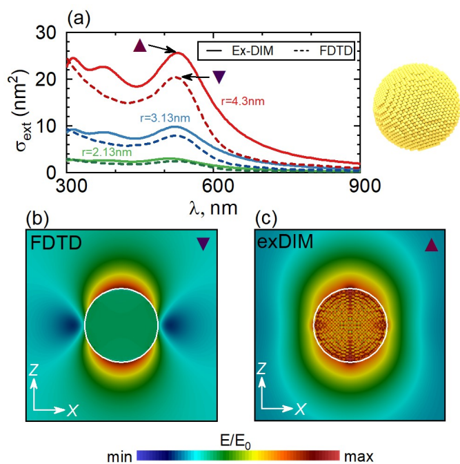
Fig. 15 Extinction cross section spectra for spherical Au nanoparticles of different sizes in aqueous medium calculated by the Ex-DIM (solid lines) and by the FDTD method (dashed lines) – (a); Configuration of local electric field calculated for spherical particle with r=4.3 nm using FDTD method – (b) and Ex-DIM – (c) for Au spherical particle at the wavelength \lambda = 525 nm. Reproduced from Ref. 152 with permission from ACS, copyright 2021.
