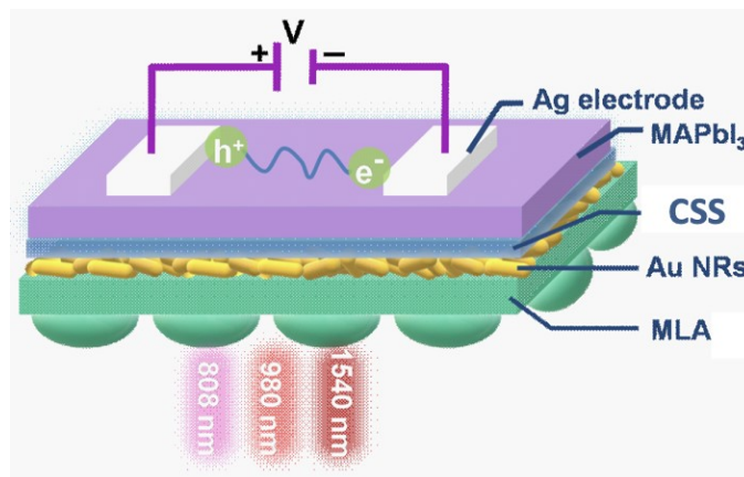
Fig. 36 Schematic illustration of a selective multispectral narrowband NIR photodetector at 808 nm, 980 nm and 1540 nm based on a hybrid structure. Reproduced from Ref. 233 with permission from Springer Nature, copyright 2020.
