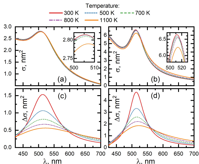
Fig. 28 Structure effect on the extinction spectra for the 6 nm Au nanoparticle from Ex-DIM calculations. Geometries are taken at different temperatures but with relaxation constant fixed at the room temperature — \Gamma_i(T = 300\text{ K}) . Insets show the enlarged fragments of spectral curves near the surface plasmon resonance maximum. Plasmonic absorption spectra of the 6 nm Au nanoparticle with subtracted interband absorption band of gold at different temperatures. (a,c) — in vacuum ( n_0 = 1 ), (b,d) — in medium with a refractive index of n_0 = 1.33 . From Ref. 193
