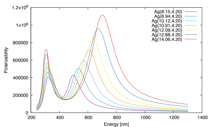
Fig. 6 Polarizability versus incident energy for Ag(x,4.20) nanorods with different longitudinal plasmon lengths. Reproduced from Ref. 75 with permission from ACS, copyright 2019.
