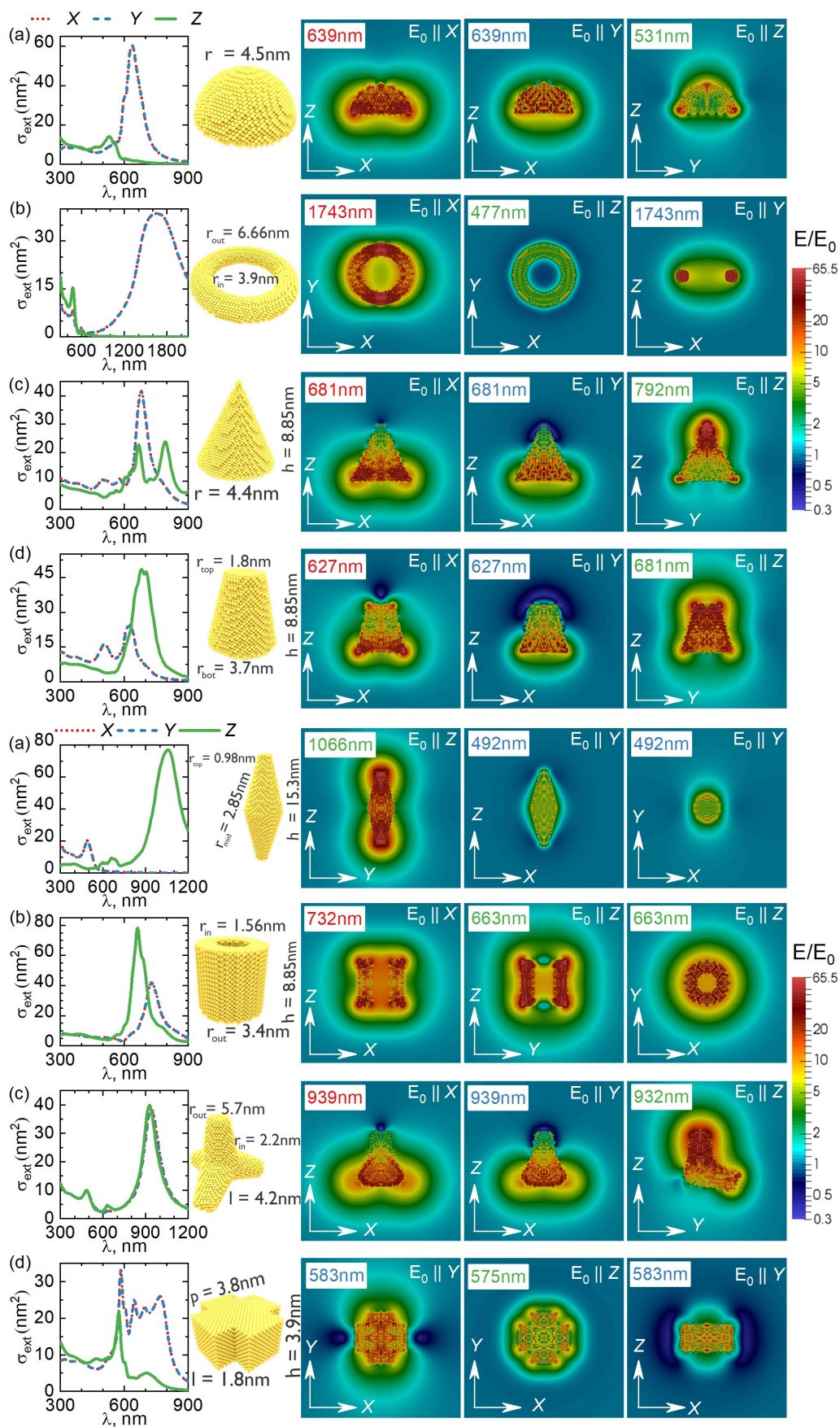
Fig. 16 Plasmonic electric fields from polarized external electric fields together spectra for ultra-fine plasmonic nanoparticles of different shape. Reproduced from Ref. 152 with permission from ACS, copyright 2021.
