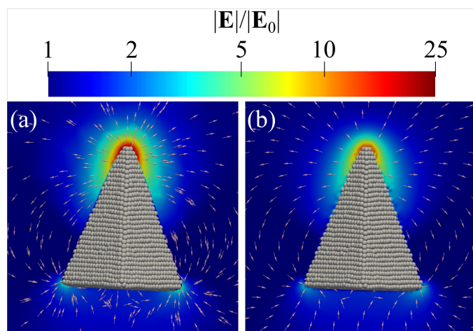
Fig. 32 Comparison of the local field distribution around a gold nanotetrahedron consisting of 26000 atoms (normalisation to the incident field strength), calculated with finite element method (COMSOL) – (a) and Ex-DIM – (b). Polarisation direction from the top to the middle of the bottom.
