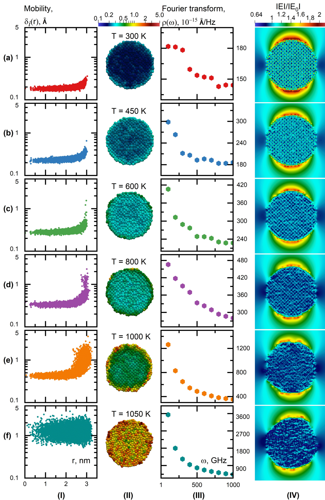
Fig. 27 Temperature dependencies (columns I, II, III, IV) of the atomic mobility in an Au nanoparticle with radius R=3 nm (I), view of this mobility in the particle cross-section with internal structure (II), the Fourier transform of the time dependent modulus of the i -th atom coordinate ( |\mathbf{r}_i(\mathbf{t})| ) as a spectral density of states in a unit range \Delta\omega_i within in the frequency range up to 10^{12} Hz (III), and distribution of the local field inside the particle and near its surface with rising temperature (for vertical polarization) (IV). From Ref. 193
