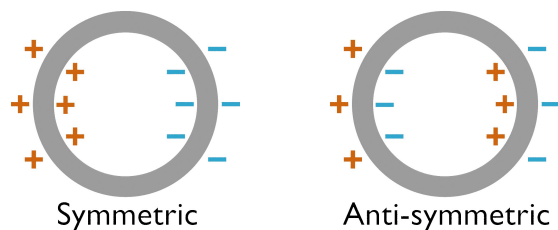
Fig. 9 Symmetrically ( \omega_- ) and an anti-symmetrically ( \omega_+ ) coupled nano-shell plasmon modes. From Ref. 143
