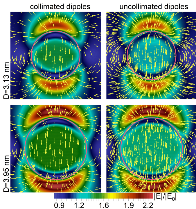
Fig. 19 The maximum field strength modulus and the field direction inside and around the Au nanoparticles with diameter 3.13 and 3.95 nm in the aqueous medium with refractive index n=1.33 at the wavelength of SPR. On the left: all dipoles in a particle are collimated, on the right: non-collimated dipoles. Polarization is vertical. Reproduced from Ref. 161 with permission from ACS, copyright 2022.
