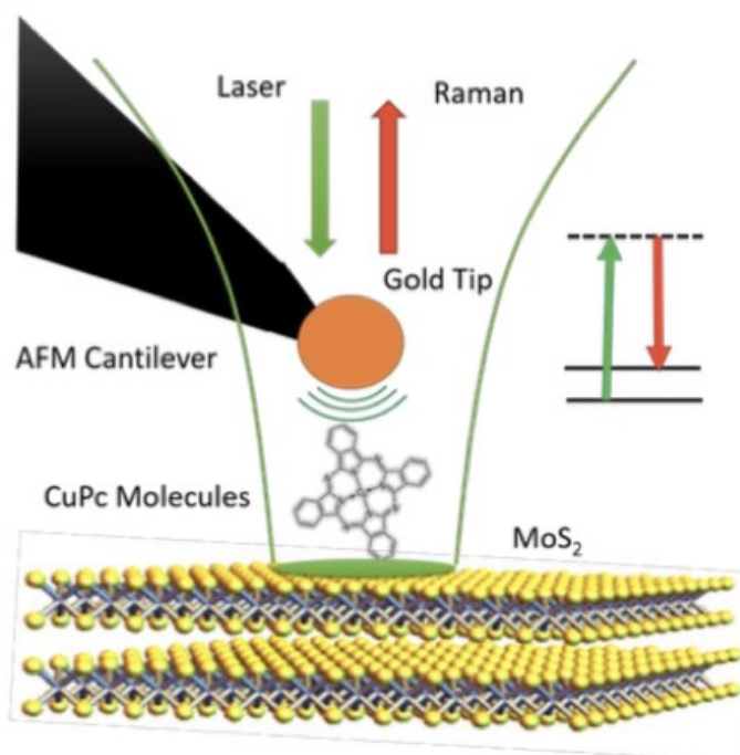
Fig. 34 Schematic overview of TERS. Reproduced from Ref. 230 with permission from IEEE, copyright 2017.
