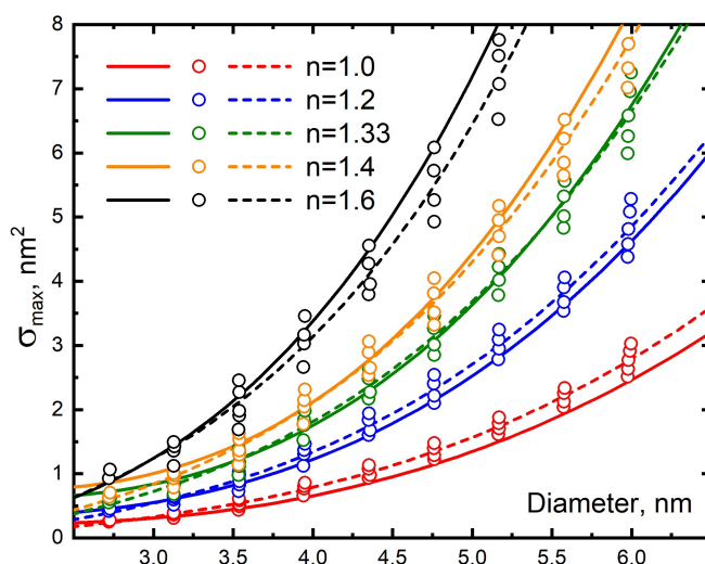
Fig. 20 Comparison of results from Mie theory and Ex-DIM model calculations of the SPR maximum as a function of Au nanoparticle size for different refractive indices of the ambient medium. Mie theory calculations obtained with size correction for the dielectric constant of Karimi 130 are given as solid lines. Discrete Ex-DIM data are given as hollow circles and approximating functions are marked as dashed lines. From Ref. 124
