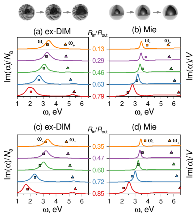
Fig. 11 Normalized imaginary polarizability from Ex-DIM model (left) and Mie theory (right) calculations for nano-shells with fixed outer radius R_{out} : 5.97 nm (top) and 7.94 nm (bottom). Squares and triangles give the positions of the symmetric ( \omega_- ) and anti-symmetric ( \omega_+ ) modes from Eq.(1) in Ref. 143 with \omega_B = 5.78 eV (Ex-DIM) and \omega_B = 6.82 eV (Mie). From Ref. 143
