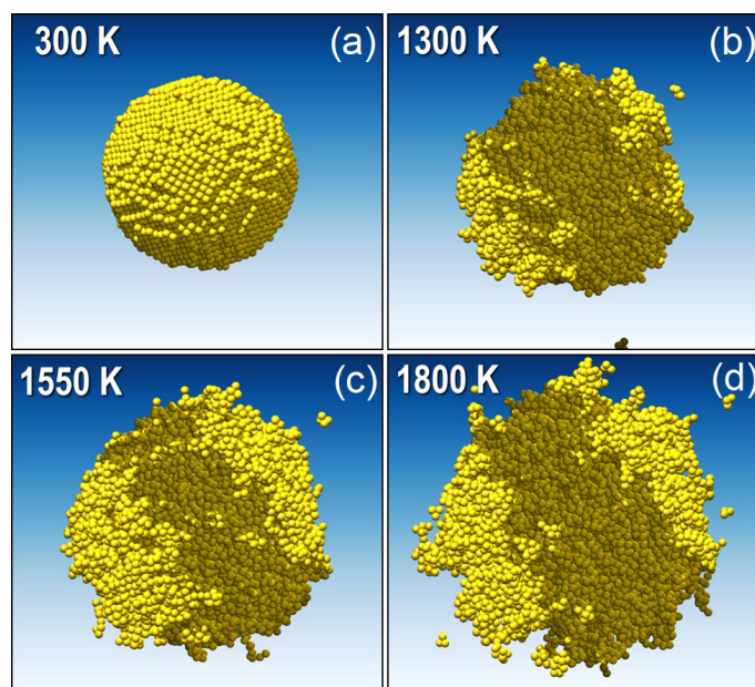
Fig. 26 Reactive force field molecular dynamics simulations of the evolution of the Au nanoparticle shape upon temperature growth – from the initial state at room temperature ( D=6 nm) directly to extremely high temperature values much above the melting point. From Ref. 193 .
