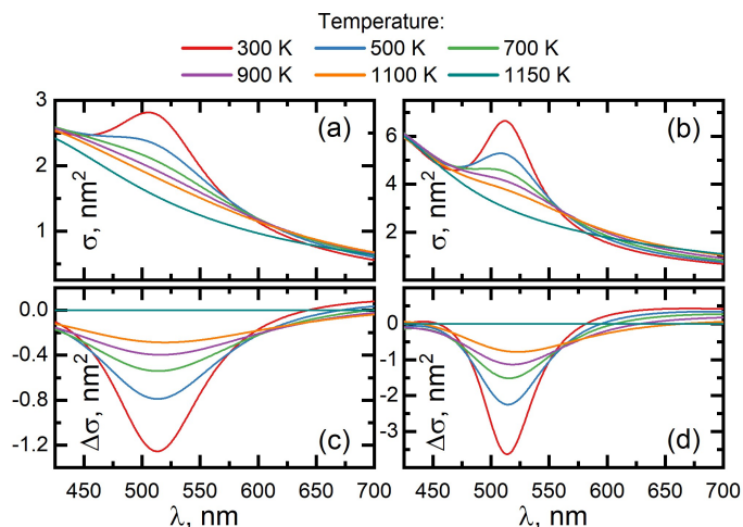
Fig. 29 Extinction spectra variation for the 6 nm Au nanoparticle with suppression of surface plasmon resonance in the temperature range 300 — 1150 K (Ex-DIM calculations). Variation of differential extinction spectra with suppression of surface plasmon resonance in for temperatures 300 — 1150 K (all curves were subtracted from the spectral dependence for T = 1150\text{ K} ). (a,b) — in vacuum, (b,d) — in medium with refractive index n_0 = 1.33 (b) From Ref. 193
