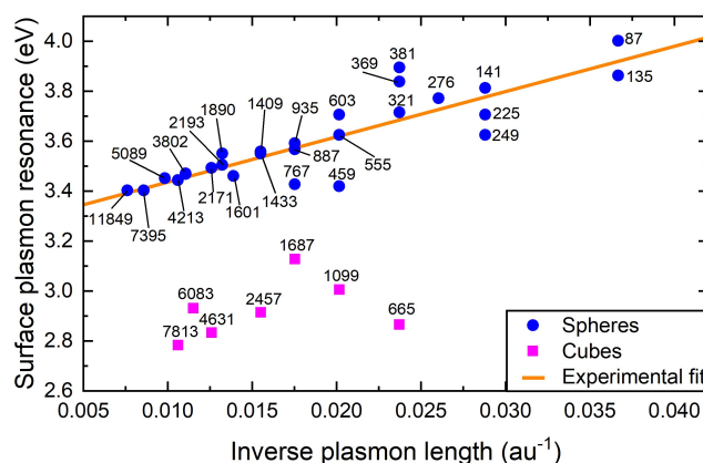
Fig. 7 SPR for sphere and cubes with different plasmon lengths. Reproduced from Ref. 75 with permission from ACS, copyright 2019.
