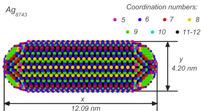
Fig. 4 Coordination numbers, longitudinal and transverse plasmon length and for an Ag nanorod containing 8743 atoms. Reproduced from Ref. 75 with permission from ACS, copyright 2019.
