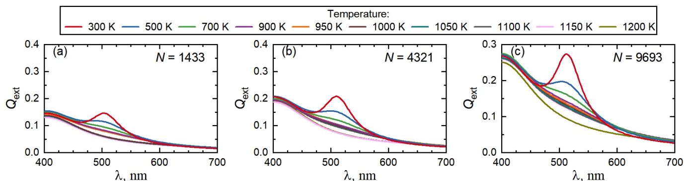
Fig. 30 The plasmonic resonance as a function of temperature for three particles with 1433, 4321 and 9693 atoms. The melting temperatures of the particles are 977 K, 1103 K and 1160 K, respectively. From Ref. 193
