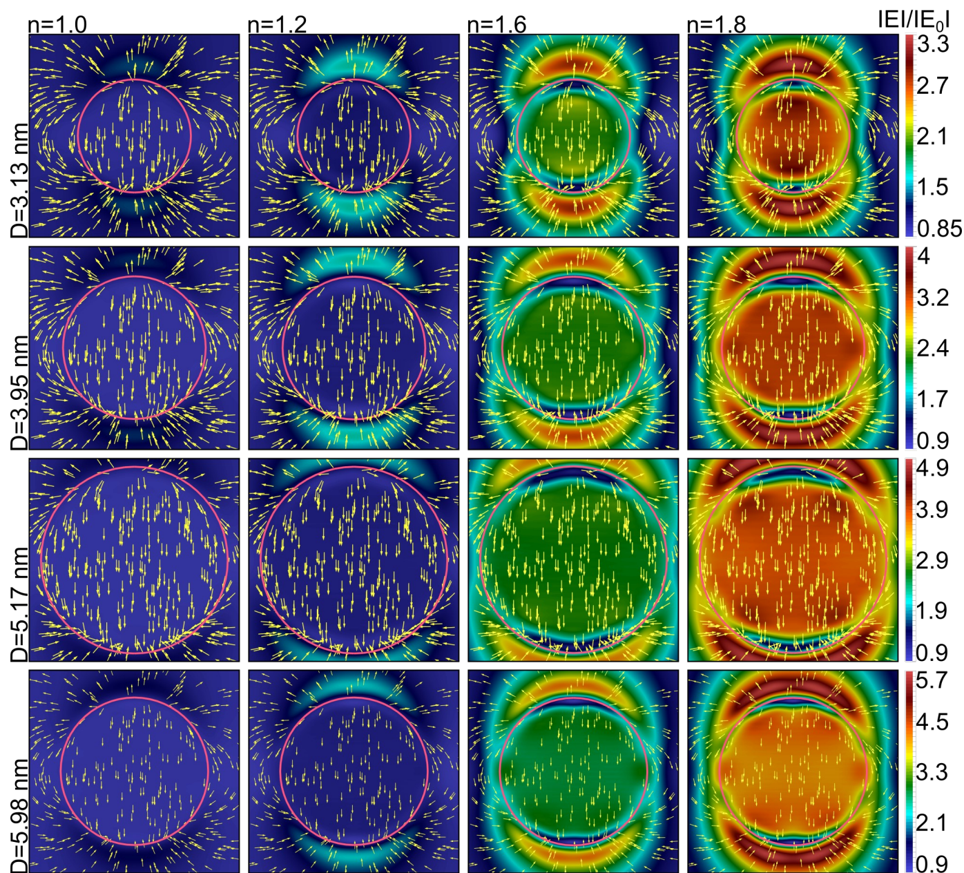
Fig. 25 Distribution of the field strength modulus ( |E|/|E_0| ) and the field directions inside and around the Au nanoparticles with diameters of 3.13, 3.95, 5.17, 5.98 nm as function of the refractive index of the ambient media n=1.0 ; 1.2; 1.6; 1.8 at the wavelength of the SPR maximum. The largest particle with a diameter of 5.98 nm with the field distribution image (in the bottom row) is reduced in order to cover the field distribution pattern around the particle. Polarization is vertical. Color bars used are different for the different sizes due to the large variation in the field amplitudes. From Ref. 124
