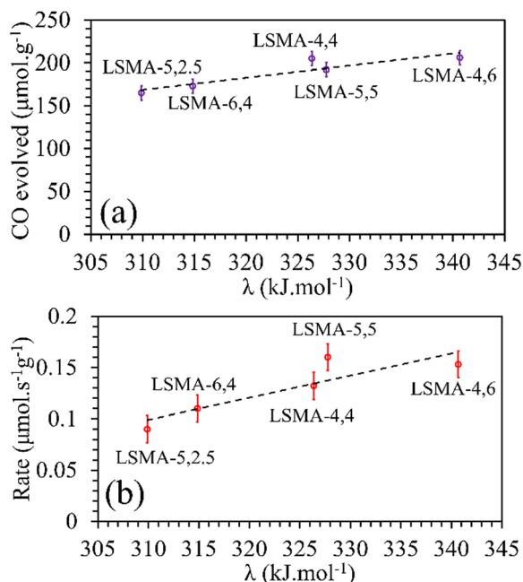
Fig. 10 Amounts of CO evolved (a) and re-oxidation rates (b) as a function of overall bond energies for a series of La x Sr 1-x Mn y Al 1-y O 3 oxygen carriers.
