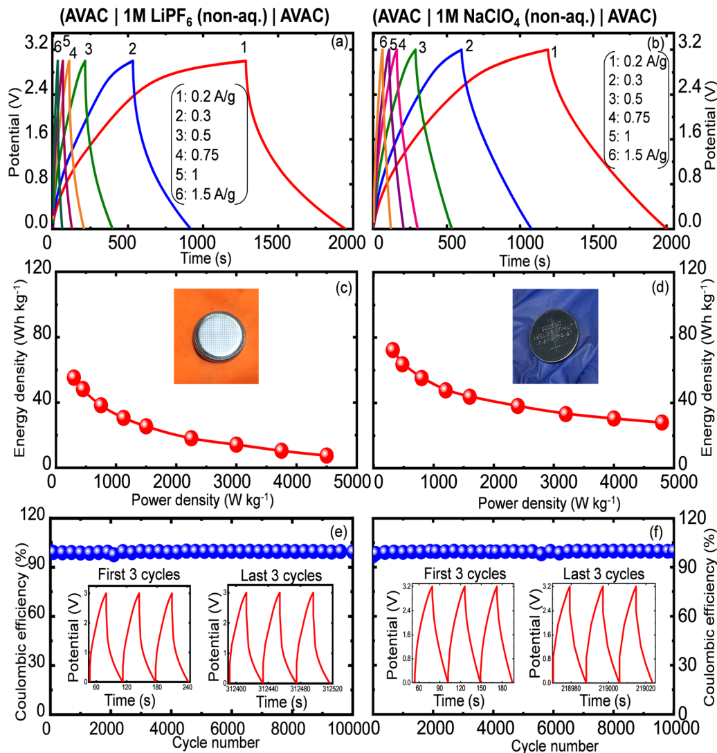
Fig. 9 (a and b) GCD curves at different currents densities for dual carbon lithium-ion capacitor (left) and dual carbon sodium-ion capacitor (right) in the CR-2032 coin cell, (c and d) Ragone plots and (e and f) Cycle life data of dual carbon lithium-ion capacitor (left) and dual carbon sodium-ion capacitor (right) in the CR-2032 coin cells in devices. Inset: First three and last three cycle charge–discharge profiles.
