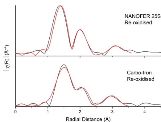
Fig. 3 U L 3 -edge Fourier transform data (black) and fits (red) for the re-oxidised NanoFeR25s and Carbo-Iron samples.
