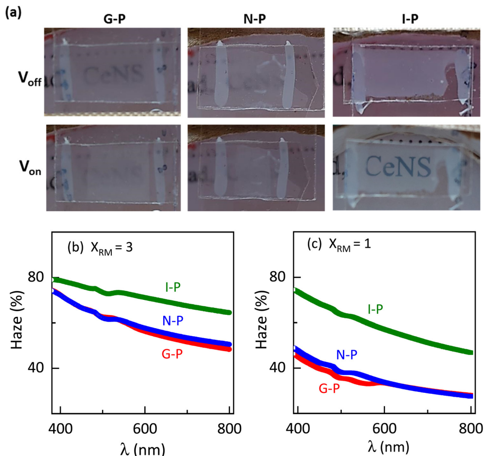
Fig. 12 (a) Images of light scattered by G-P, N-P, and I-P at room temperature for X_{RM} = 3 . Visually, we can observe higher haze for the I-P sample. Haze measured in the visible region for (b) X_{RM} = 3 and (c) X_{RM} = 1 . Higher haze is exhibited for X_{RM} = 3 . I-P samples scatter more light compared to G-P and N-P for both X_{RM} = 3 and 1.
