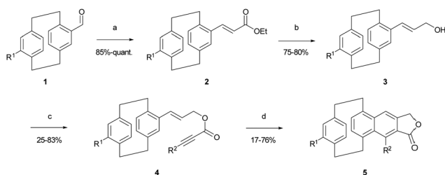
Scheme 3 Synthesis of pCp-based naphthalenes. Reaction conditions: (a) triethyl phosphonoacetate (1.5 equiv.), DBU, Ar, rt, 4 h; (b) DIBAL-H (4 equiv.), Et 2 O, Ar, -78^\circ \text{C} to rt, 4 h; (c) propiolic acid derivative (1.05 equiv.), DCC (1 M in CH 2 Cl 2 , 1.5 equiv.), DMAP (0.01 equiv.), CH 2 Cl 2 , Ar, rt, 4 h; (d) \mu\text{w} , PhNO 2 , 180^\circ \text{C} , 30 min.
