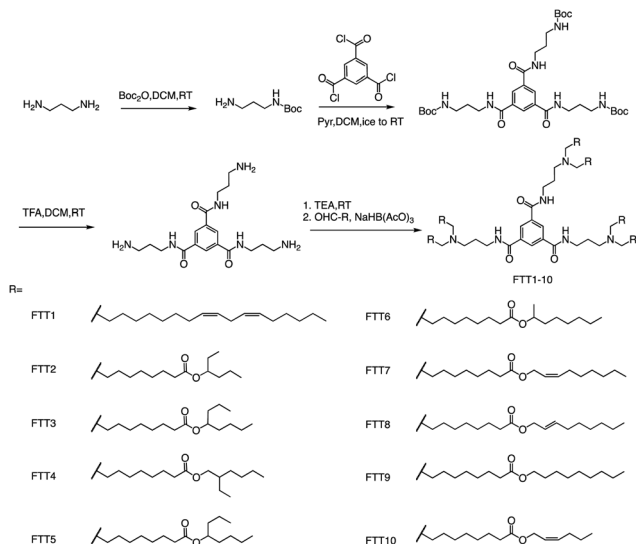
Fig. 7 The general method for synthesizing FTT1-10. Abbreviations: di- t -butyl decarbonate (Boc 2 O), pyridine (Pyr), and sodium triacetoxyborohydride is NaBH(OAc) 3 .
