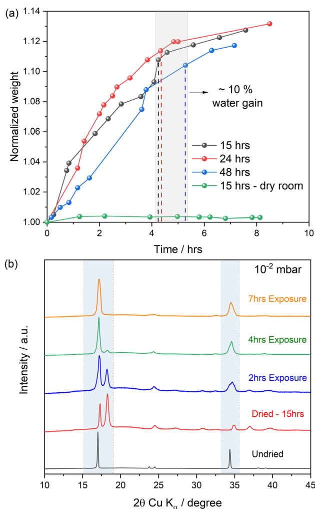
Fig. 3 Moisture exposure test for PW powders previously dried for 15, 24 and 48 hours and subsequently exposed to moisture in standard lab environment and dry room condition. (a) Weight gain (water adsorption) upon time. (b) XRD patterns of sample exposed to moisture for 2, 4, 7 hours compared with pristine monoclinic powder and sample dried for 15 hours.
