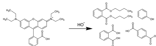
Fig. 11 Proposed mechanisms of initial degradation steps of (a) EB, (b) MO, (c) MB and (d) RhB by hydroxyl radicals.
