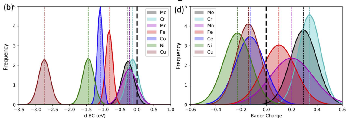
Fig. 5 Normal distribution of the d BC (a and b) and Bader charges (c and d) of the adsorbing elements of the 556 randomly created microstructures. Here, elements placed on the subsurface and surface of the microstructures are differentiated. Surface elements are accounted for in (a) and (b), while subsurface atoms are considered in (b) and (d). Subsurface atoms are the referent elements on the second layer of the slab from top to bottom.
