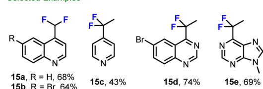
Scheme 4 Catalyst free late-stage C–H monofluorination and difluorination of heterobenzylic C–H bonds.
