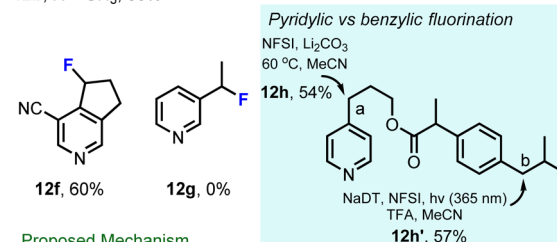
Scheme 3 (a) Decatungstate-catalyzed and AIBN-initiated fluorination of benzylic C–H bonds. (b) Decatungstate-catalyzed synthesis of acyl fluorides from aldehydes. Image reproduced with permission from ref. 58, copyright 2015 the Royal Society of Chemistry.
