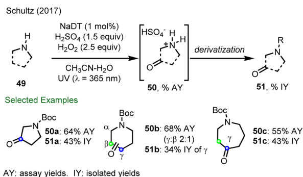
Scheme 13 Decatungstate catalyzed C–H oxyfunctionalization of the remote C–H bonds of aliphatic amines and the observation of site-selective C–H oxidation. AY: assay yields by ^1\text{H} NMR analysis; IY: yields of isolated products.
