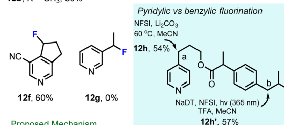
Scheme 3 (a) Decatungstate-catalyzed and AIBN-initiated fluorination of benzylic C–H bonds. (b) Decatungstate-catalyzed synthesis of acyl fluorides from aldehydes. Image reproduced with permission from ref. 58, copyright 2015 the Royal Society of Chemistry.
