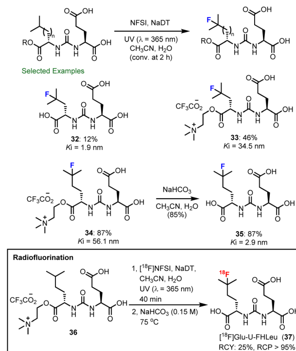
Scheme 9 Accelerated fluorination of choline esters of ZJ-43 and Glu-U-HLeu. PSMA binding of each ligand ( K_i ) was measured by competition assays ( n \geq 3 ) using [ ^{18}\text{F} ]DCFPyL and determined by applying a one-site Fit K_i model using GraphPad Prism (7.04).
