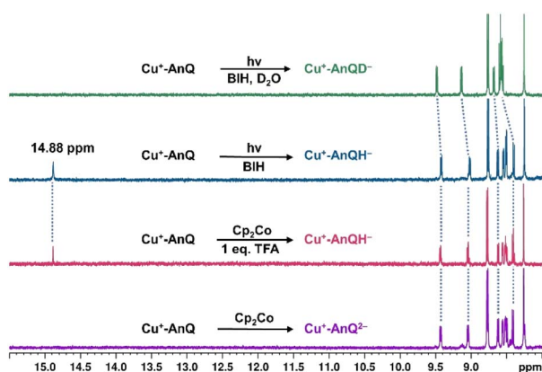
Fig. 7 Comparison of the ^1\text{H} NMR spectra of \text{Cu}^+\text{-AnQ}^{2\cdot-} (purple line), \text{Cu}^+\text{-AnQH}^\bullet generated by \text{Cp}_2\text{Co} and 1 eq. trifluoroacetic acid (red line), \text{Cu}^+\text{-AnQH}^\bullet generated by 30 minutes illumination with BIH (teal line), \text{Cu}^+\text{-AnQD}^{\cdot-} generated by BIH with 30 min illumination and then added with one drop of \text{D}_2\text{O} (green line). Illumination with 455 nm light; concentrations of the complex and BIH were kept at 0.2 mM and 0.1 M, respectively, in \text{CD}_3\text{CN} .
