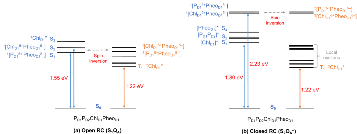
Fig. 8 Schematic representation of the singlet and triplet vertical excitation energies of the P_{D1}P_{D2}Chl_{D1}Pheo_{D1} tetramer in: (a) the open RC ( S_1Q_A ), and (b) the closed RC ( S_2Q_A^- ). All energies are reported relative to the ground state singlet ( S_0 ).
