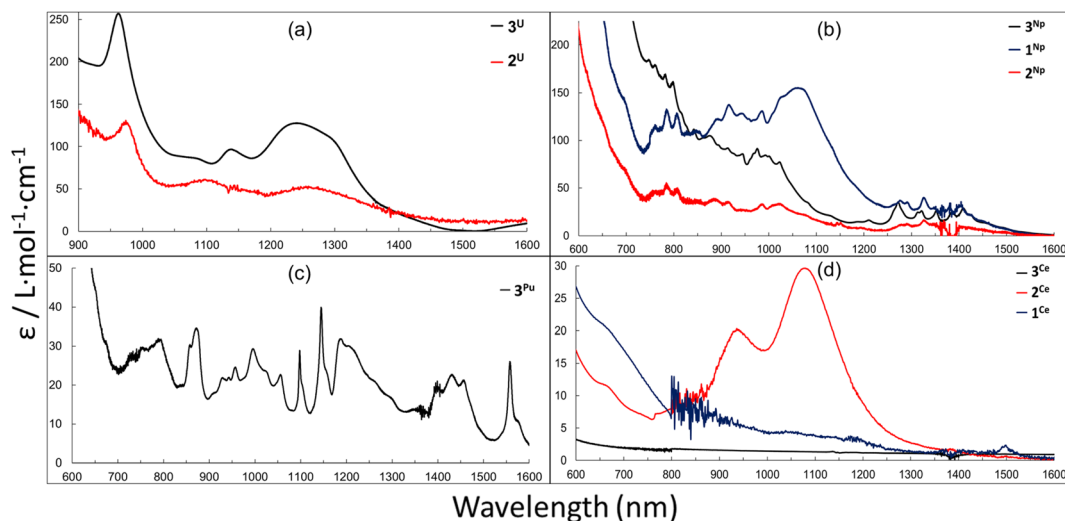
Fig. 5 (a): NIR spectra for 2^{\text{U}} (4.6 mM in Tol) and 3^{\text{U}} (3.0 mM in THF). (b): vis-NIR spectra for the 1^{\text{Np}} , 2^{\text{Np}} and 3^{\text{Np}} series. (0.69 mM in Tol, 0.50 mM in Tol and 2.1 mM in THF respectively). (c): vis-NIR spectra for 3^{\text{Pu}} (1.0 mM in THF). (d): vis-NIR spectra of 3^{\text{Ce}} , 2^{\text{Ce}} and 1^{\text{Ce}} (9.51 mM, 5.86 mM and 2.32 mM respectively) in toluene.
