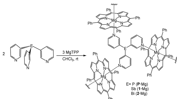
Scheme 2 Synthesis of the complexes \{[\text{P}(3\text{-py})_3]_2 \cdot (\text{MgTPP})_3\}_n ( \text{P} \cdot \text{Mg} ), \{[\text{Sb}(3\text{-py})_3]_2 \cdot (\text{MgTPP})_3\}_n ( 1 \cdot \text{Mg} ) and \{[\text{Bi}(3\text{-py})_3]_2 \cdot (\text{MgTPP})_3\}_n ( 2 \cdot \text{Mg} ).
