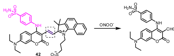
Fig. 18 Reaction-based detection mechanism of probe 42 for ONOO − .
