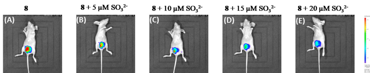
Fig. 9 In vivo photos of nude mice (A) 8 (20 μM); (B–E) 8 (20 μM) + different concentrations of SO 3 2- (5–20 μM). \lambda_{\text{ex}} = 530 nm, \lambda_{\text{em}} = 600–700 nm. Reprinted from ref. 88, copyright 2021 Elsevier.
