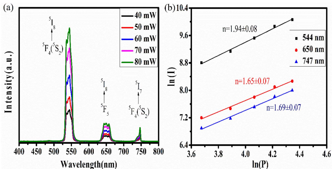
Fig. 6 (a) The power-dependent upconversion spectra and (b) the double logarithmic plot for calculation of the number of photons.
