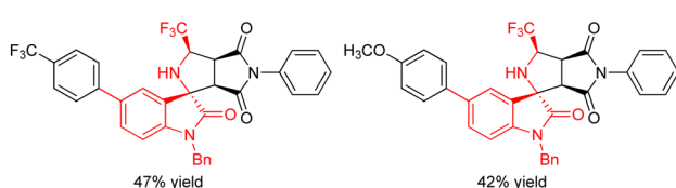
Scheme 6 Phase transfer-catalyzed stereoselective formation of spiro-fused[succinimide-pyrrolidine-oxindoles].
