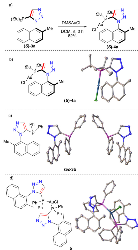
Fig. 3 (a) Synthesis of a single enantiomer gold(i) chloride complex (b) single-crystal X-ray diffraction structure of (S) - 4a . Ellipsoids are drawn at the 50% probability level. A molecule of DCM has been omitted for clarity. Hydrogen atoms omitted for clarity. (c) Molecules from the crystal structure of rac - 3b with ellipsoids drawn at the 50% probability level. Symmetry codes used to generate the equivalent atoms: (i) x, y, z , (ii) 1 - x, 1 - y, 1 - z . Hydrogen atoms omitted for clarity. (d) Single-crystal X-ray diffraction structure of homo-chiral complex 5 . Ellipsoids are drawn at the 50% probability level. A molecule of DCM has been omitted for clarity. Hydrogen atoms have been omitted for clarity.
