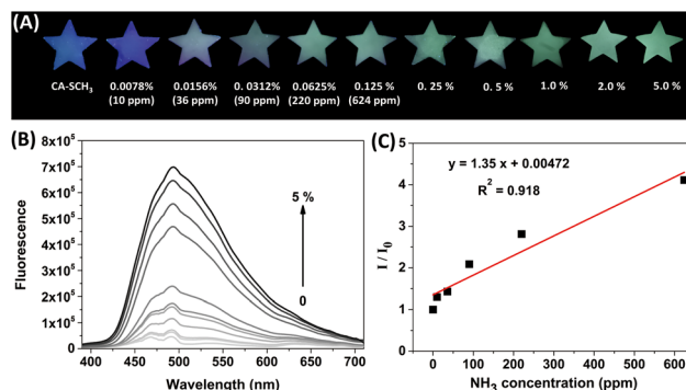
Fig. 3 (A) Photographs of paper-based sensor CA-SCH 3 treated with various concentrations of \text{NH}_3\cdot\text{H}_2\text{O} for 1 h were taken under UV light (365 nm). (B) Solid state fluorescence spectra of the filter papers in (A). (C) Linear fitting of I/I_0 with ammonia concentrations ranging from 0 to 624 ppm. I_0 and I show the fluorescence intensities of CA-SCH 3 at 495 nm and that upon exposure to various concentrations of amine vapor.
