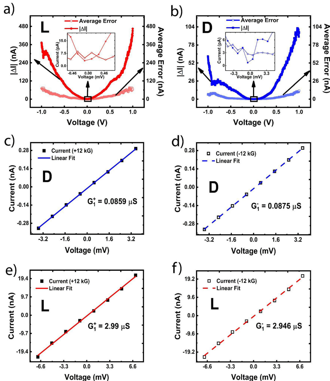
Fig. 3 (a and b) CISS signal magnitude |\Delta I| as a function of bias ( V ) for L and D functionalized samples, respectively. Average error for the current measurements has also been plotted in each case. CISS signal magnitude |\Delta I| increases with bias, but as shown in the insets, in the vicinity of zero bias, it falls below the noise floor. (c and d) Linear range conductance measurements for D functionalized samples for \pm 12 kG. The values are nominally identical, considering the noise margin in this bias range. (e and f) Linear range conductance measurements for L functionalized samples for \pm 12 kG. The values are nominally identical, considering the noise margin in this bias range.
