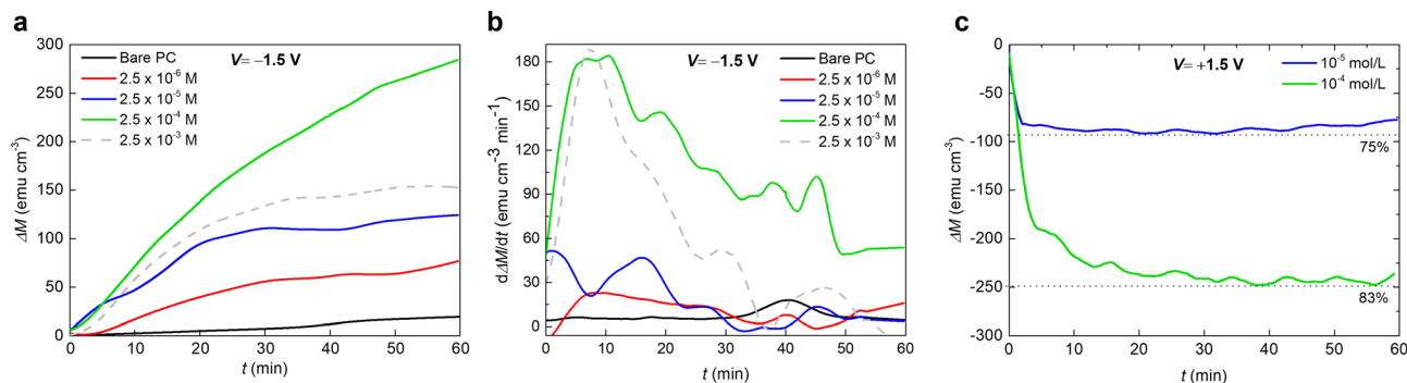
Fig. 3 Impact of KI concentration in PC on Co oxide magneto-ionics. (a) Magnetization ( \Delta M ) as a function of time t for PC with different KI concentrations under electrolysing at -1.5 V, while applying an external in-plane magnetic field of 10 kOe, and (b) the respective magneto-ionic rate, d\Delta M/dt . (c) Magnetization ( \Delta M ) depletion as a function of time t for the two best performing KI concentrations under an opposite bias ( +1.5 V), while applying an external in-plane magnetic field of 10 kOe.
