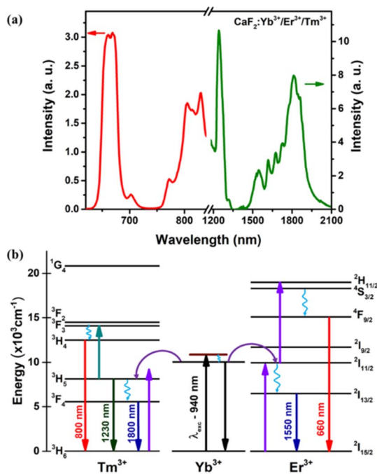
Fig. 5 (a) Emission spectrum of \text{Yb}^{3+}/\text{Er}^{3+}/\text{Tm}^{3+} tri-doped \text{CaF}_2 NPs under 940 nm excitation at room temperature in the I-BW (red), II-BW (left peak of the green spectrum) and III-BW (right peak of the green spectrum). (b) Simplified energy scheme of the \text{Yb}^{3+} , \text{Er}^{3+} and \text{Tm}^{3+} ions, showing excitation and emission decays (full lines), nonradiative decays (wavy lines), and the energy transfer process (curved lines).
