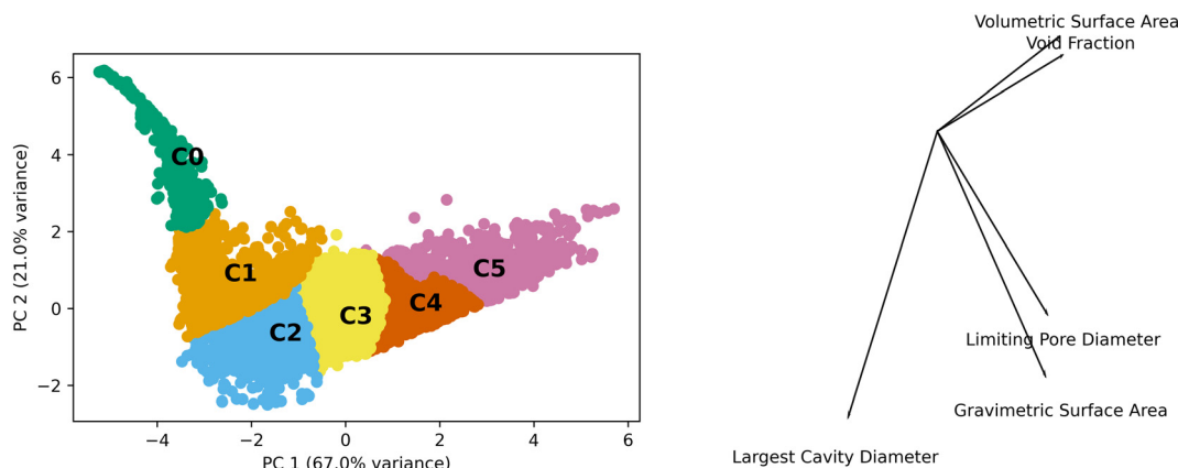
Fig. 2 Clustering in principal component space. The left panel shows the top two principal components and how the space was clustered. The right panel shows a biplot revealing how the different features are represented in the principal components.
