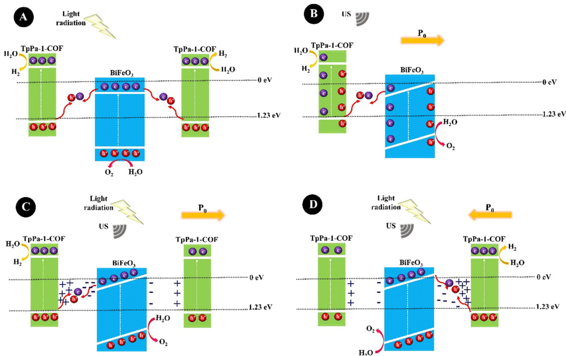
Fig. 4 The representative diagrams of photocatalysis (A), piezocatalysis (B), and piezo/photocatalysis (C) and (D) for \text{BiFeO}_3@ \text{TpPa-1-COF} (adapted from ref. 162 with permission from John Wiley and Sons).
